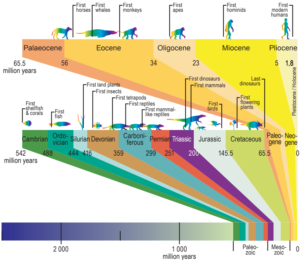
The Geological Timescale
