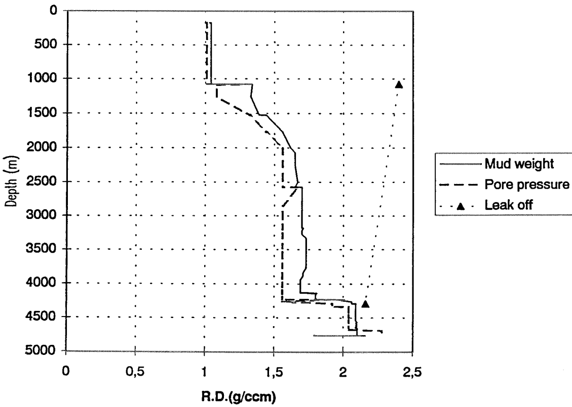
Composite plot for well: 2/7-23 S
