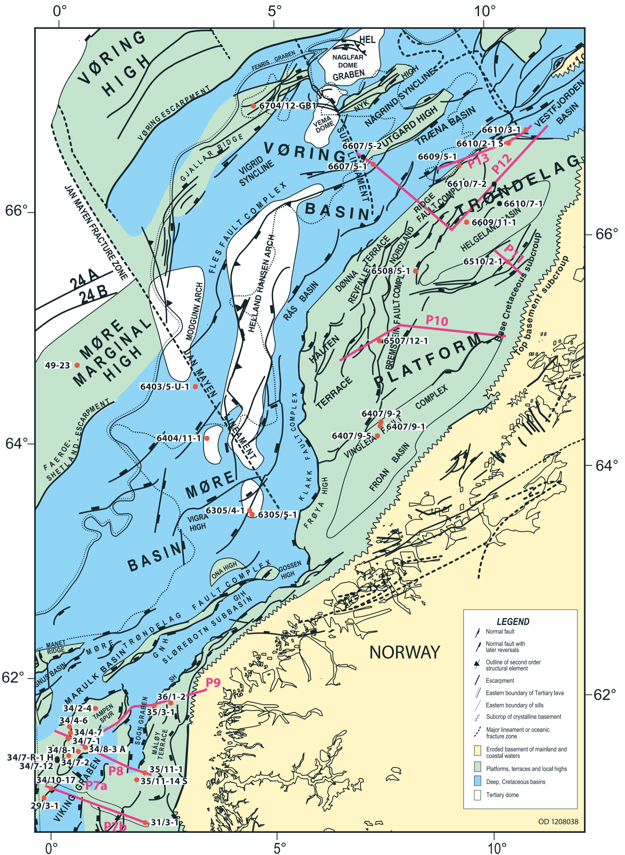
Fig. 6: Map showing structural elements and seismic lines in the Norwegian Sea, on the Norwegian Sea continental shelf and in the northernmost part of the North Sea (modified after Brekke 2000). Red dots are investigated wells and boreholes, black dots are wells and boreholes referred to and magenta lines are locations of seismic profiles.
