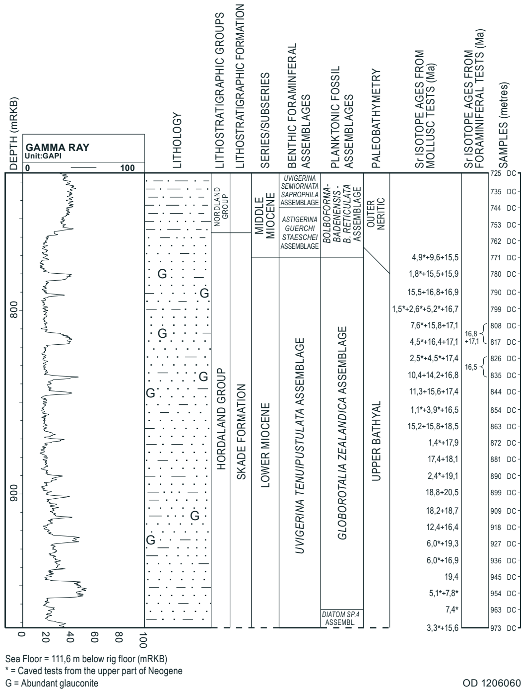
Fig. 2: Well summary figure including gamma ray log, lithology, lithostratigraphic units, series/subseries, benthic foraminiferal assemblages, planktonic fossil assemblages, paleobathymetry, strontium isotope ages and analysed samples for the middle part of the investigated sequence in well 25/10-2 (Lower to Middle Miocene, modified after Eidvin & Rundberg 2007).
