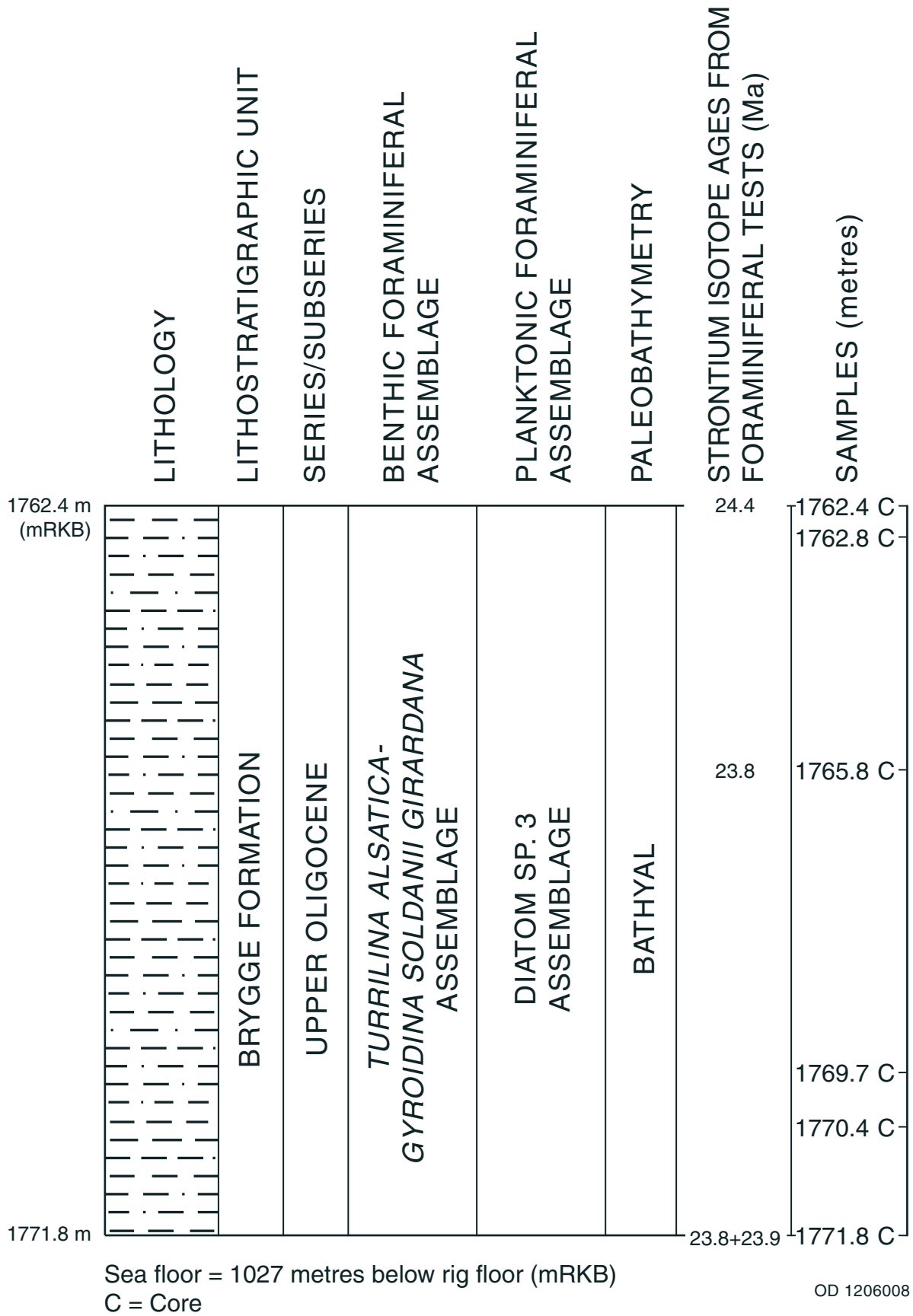
Fig. 1: Well summary figure for the cored Oligocene section in well 6305/4-1 including lithology, lithostratigraphic unit, series/subseries, benthic foraminiferal assemblage, planktonic fossil assemblage, paleobathymetry, strontium isotope ages and analysed samples.
